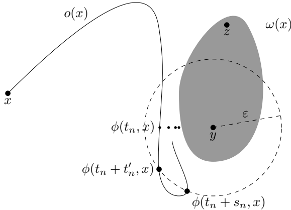
RYSUNEK 1. Sketch of the proof of Lemma 3.3.
