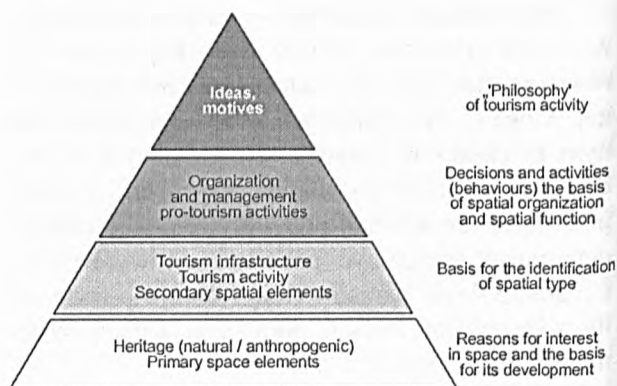
Fig. 10. Levels of research into tourism space (source: author)
