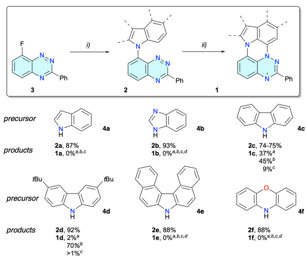
Scheme 1 Synthesis of benzo[e][1,2,4]triazines 2 and their photocyclization to radicals 1 at c ≈ 1 mM. a Reagents and conditions: (i) heteroarene 4a–4f , 60% NaH, dry DMSO, 80 °C, 3 h; (ii) 300 W halogen lamp in a Pyrex flask, 1 mM (a) in CH 2 Cl 2 , (b) in EtOAc or (c) in EtOH, 30–35 °C, 72 h; (d) no reaction.
