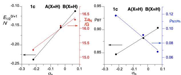
Fig. 13 Left: correlation of E_{1/2}^{0/+1} (black) and the sum of hfcc a_N for the triazine ring (red) with Hammett parameters \sigma_p for −SPh (0.07), −OPh, (−0.03) and −NPh 2 , (−0.22). Right: correlation of DFT spin density for the benzo[e][1,2,4]triazine ring ( \rho_{BT} , black) and for the benzene ring at the N(1) position of the triazine ( \rho_{N1Ph} , blue) with \sigma_p .
